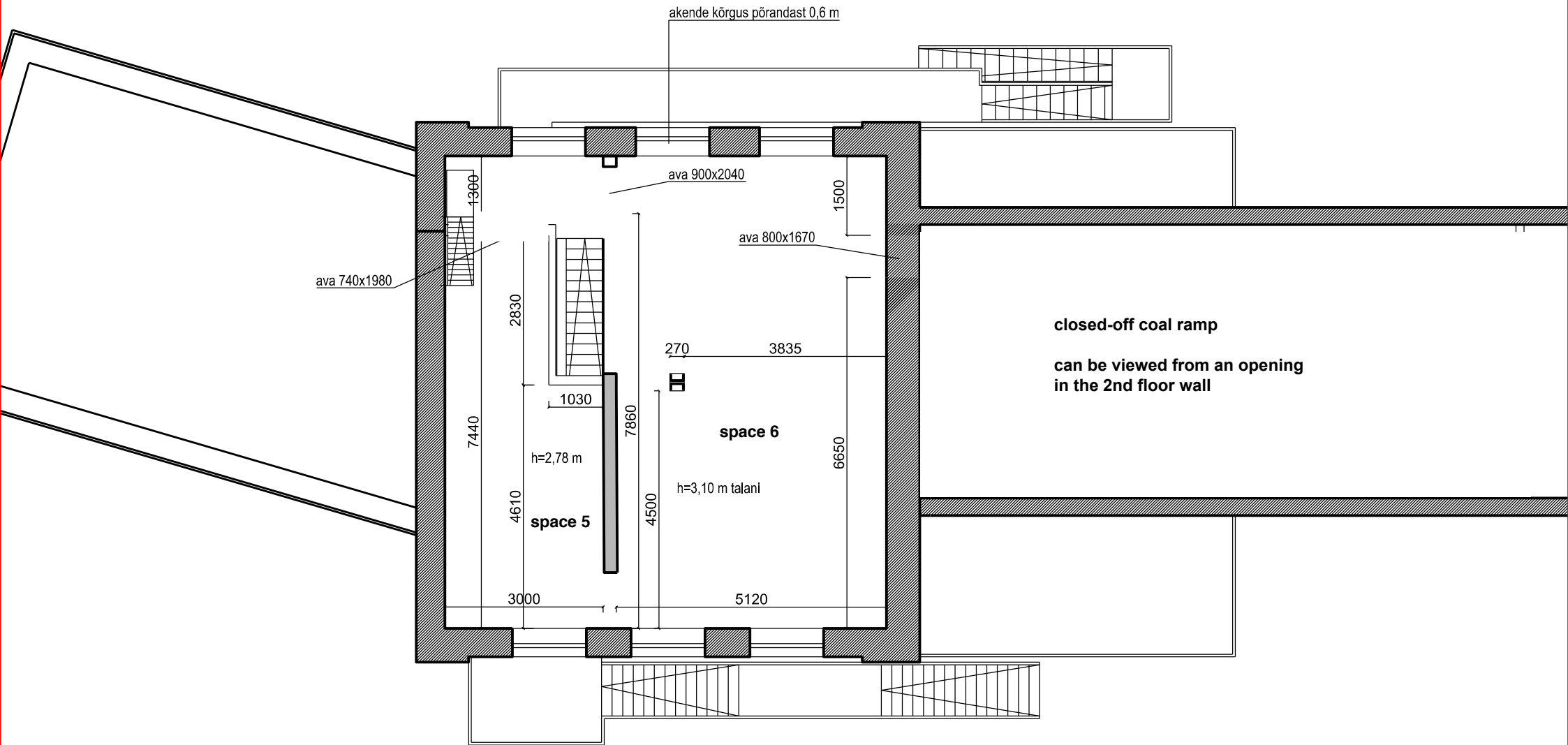
EKKM 2nd FLOOR M1:100
