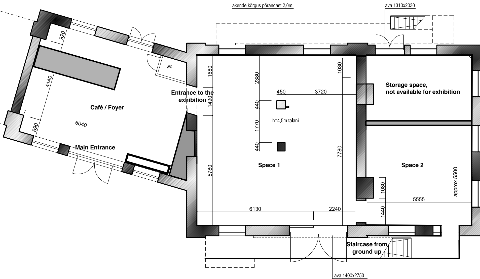
EKKM GROUND FLOOR M 1:100
